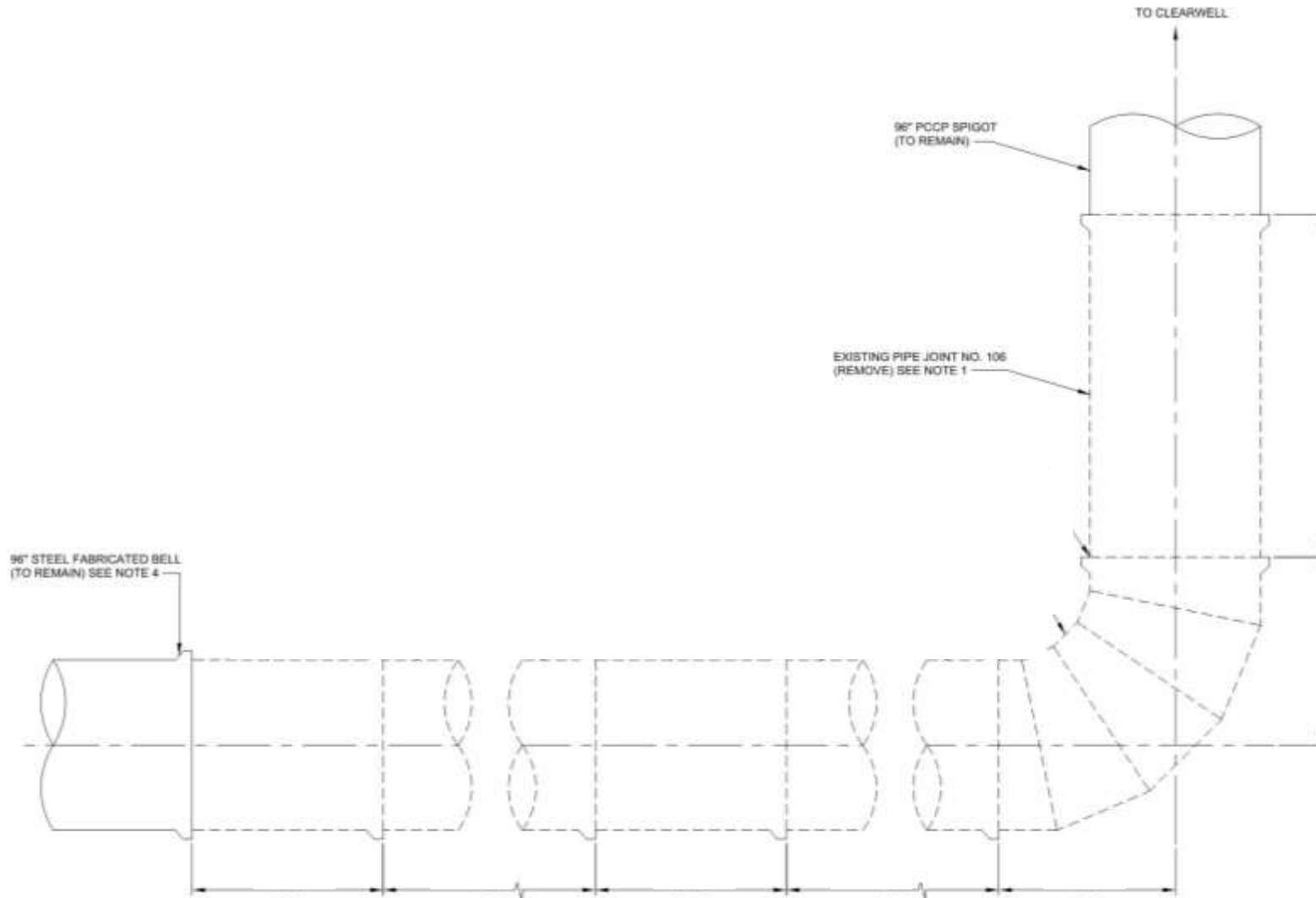
A EXISTING CLEARWELL BYPASS 96" PCCP PIPE
